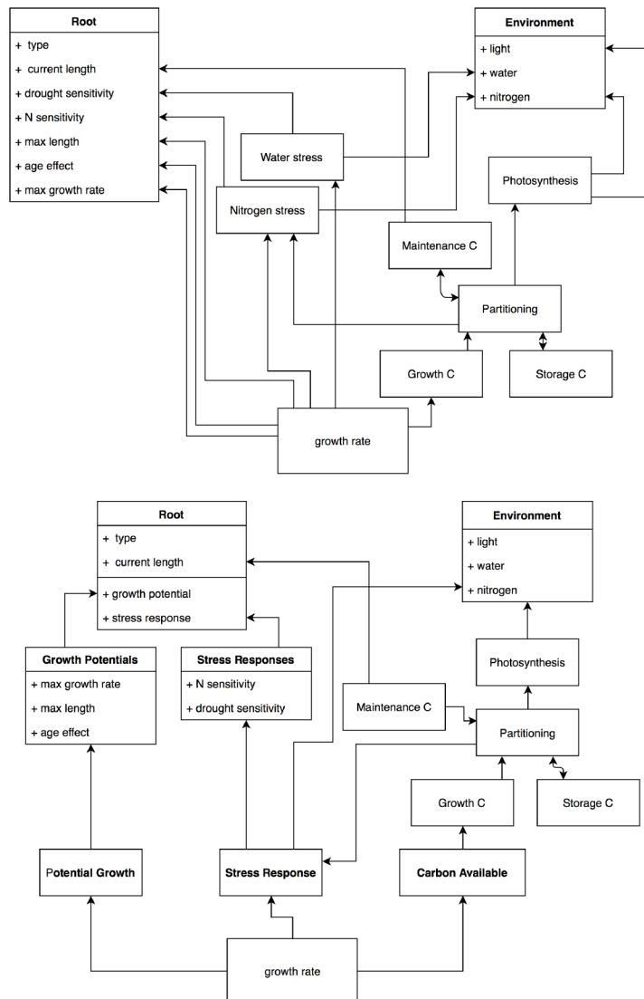
1005 Figure 5: Conceptual diagrams illustrating "loose" vs "tight" coupling between model 1006 components. Shown are two possible implementations of a hypothetical model calculating the 1007 elongation of a single root based on assimilate supply, genetic potential, and carbon 1008 partitioning factors. Each box represents a group of related calculations or values (which 1009 would likely be implemented as a class), and arrows indicate information lookup (e.g. read x - 1010 > y as "x uses y"). Top panel: Tightly coupled design. Each calculation requires detailed 1011 knowledge of the internal details of other modules. Bottom panel: Loosely coupled design. 1012 Modules share information through standardized interfaces "Potential Growth", "Stress 1013 Response", and "Carbon Available", thus isolating the growth rate calculation from the details 1014 of e.g. where and how parameters are stored or whether the potential growth rate of the 1015 current root is limited more by developmental factors or by root type parameters. Note that 1016 both implementations ultimately perform the same set of calculations; thoughtful code design 1017 can improve maintainability and interoperability even within a set mathematical framework.
